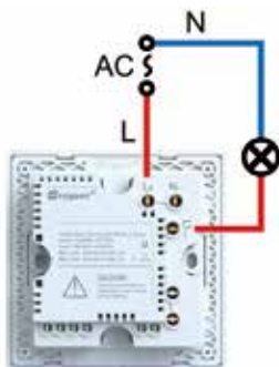
Connection 1: Without neutral wire
