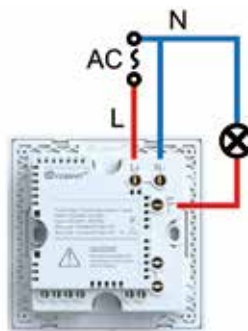
Connection 2: With neutral wire
